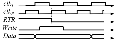
Fig 2. Handshaking in GALS
