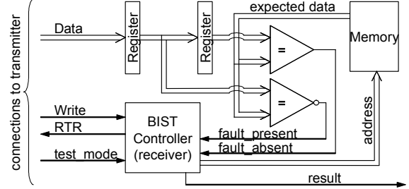
Fig 4. Receiver
