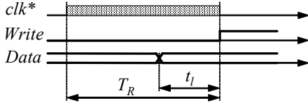
Fig 3. Timing diagram of extra reading
